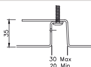
Slimwall CPS-SSF-S ; module 250mm to 1000mm
